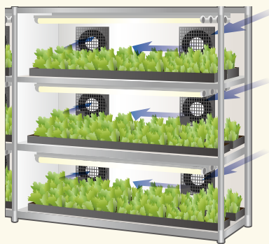
Air circulation (Inside showcases, in plant factories, etc.)
