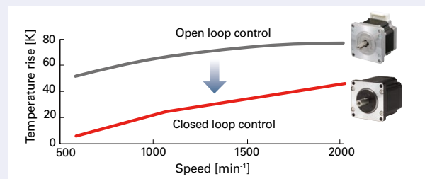
Motor temperature rise
