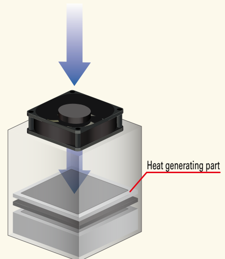
Cooling by blowing
